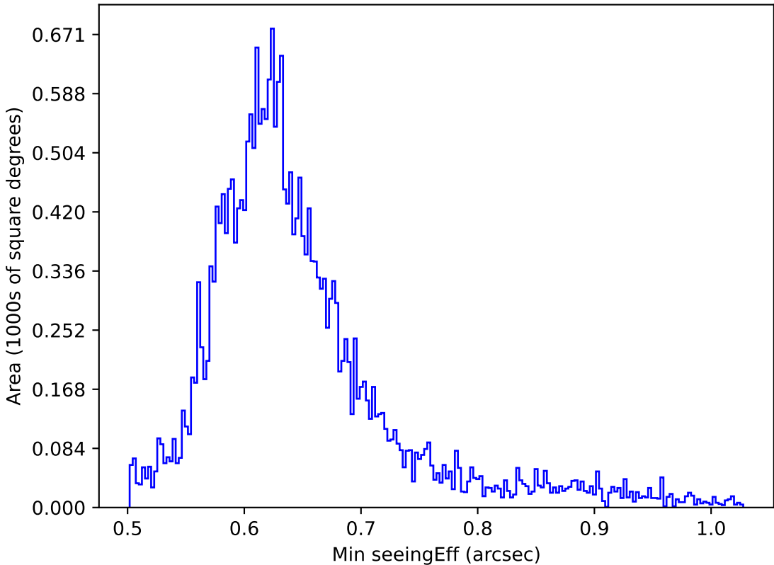
too_elab_r128_d3_ugrizy_v3.4_10yrs All sky z band: Min seeingEff
