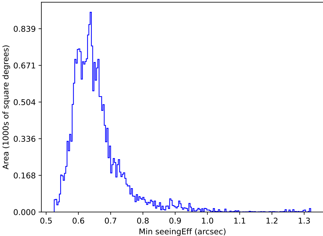
too_elab_r128_d3_ugrizy_v3.4_10yrs All sky y band: Min seeingEff
