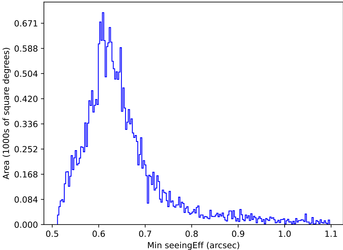
too_elab_r128_d3_ugrizy_v3.4_10yrs All sky r band: Min seeingEff
