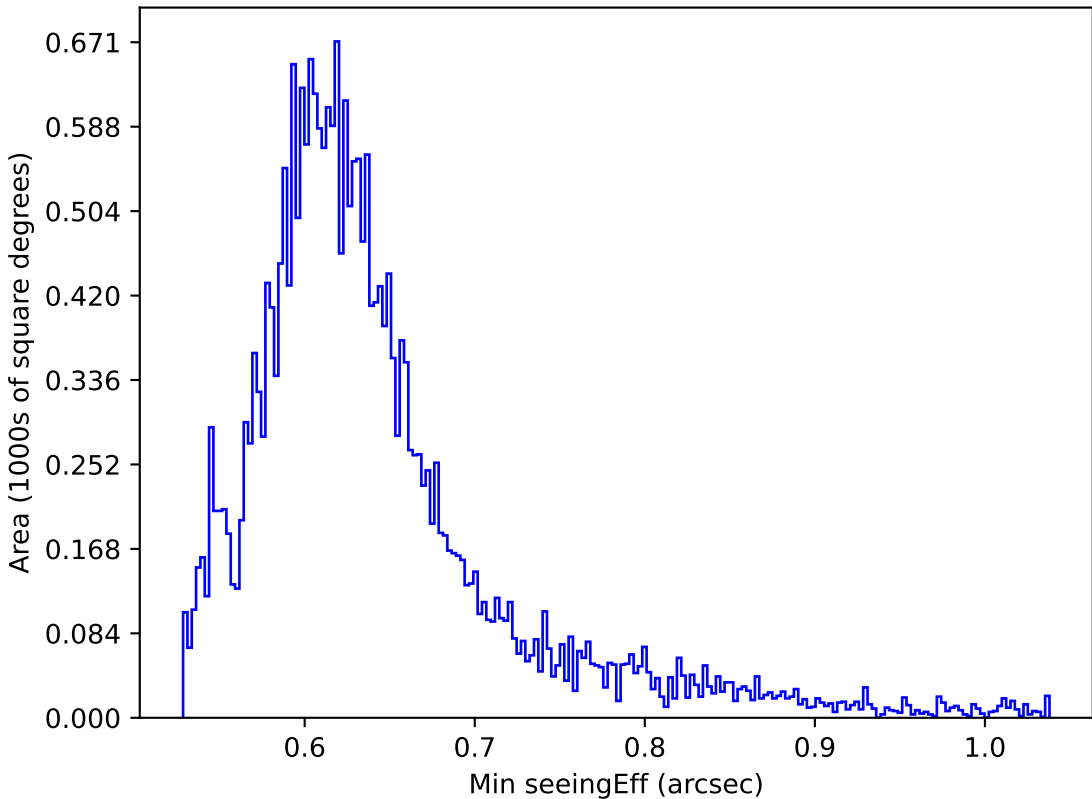
too_elab_r128_d3_ugrizy_v3.4_10yrs All sky i band: Min seeingEff
