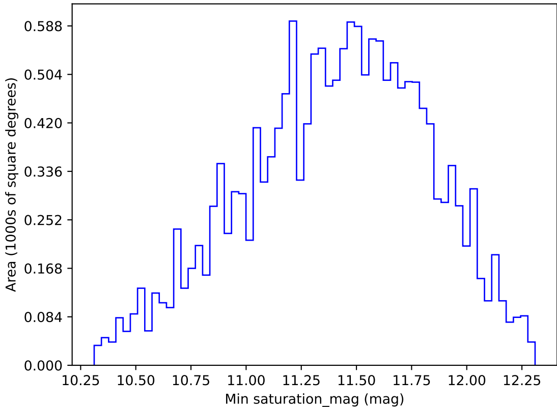
too_elab_r128_d3_ugrizy_v3.4_10yrs WFD u band: Min saturation_mag
