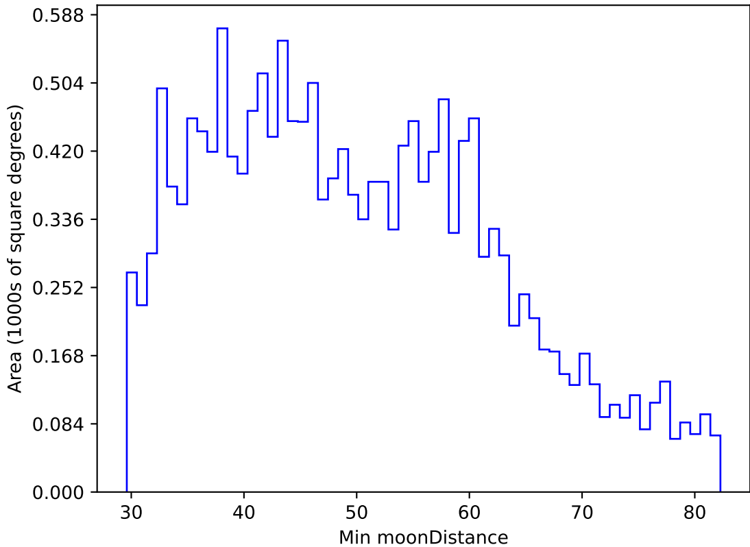
too_elab_r128_d3_ugrizy_v3.4_10yrs WFD u band: Min moonDistance
