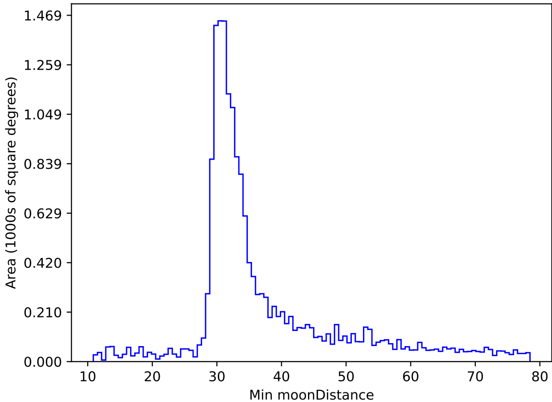
too_elab_r128_d3_ugrizy_v3.4_10yrs WFD r band: Min moonDistance
