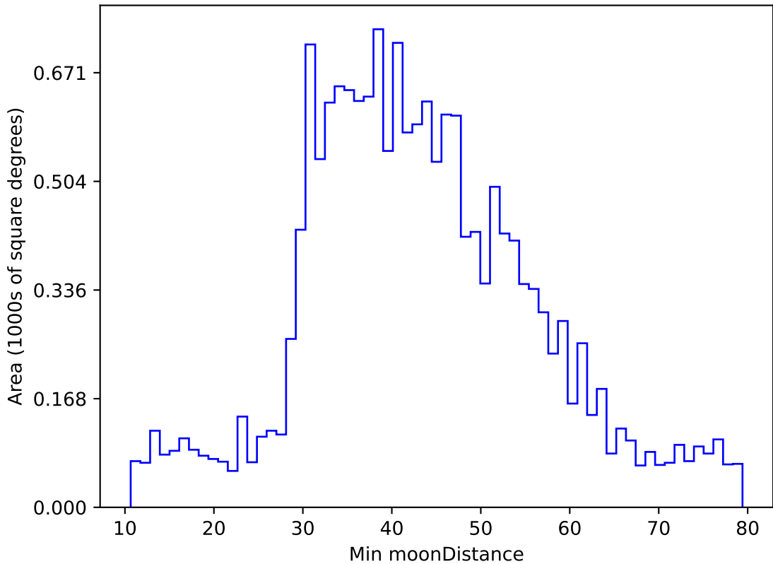
too_elab_r128_d3_ugrizy_v3.4_10yrs WFD g band: Min moonDistance
