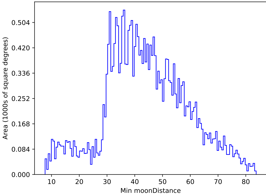
too_elab_r128_d3_ugrizy_v3.4_10yrs All sky g band: Min moonDistance
