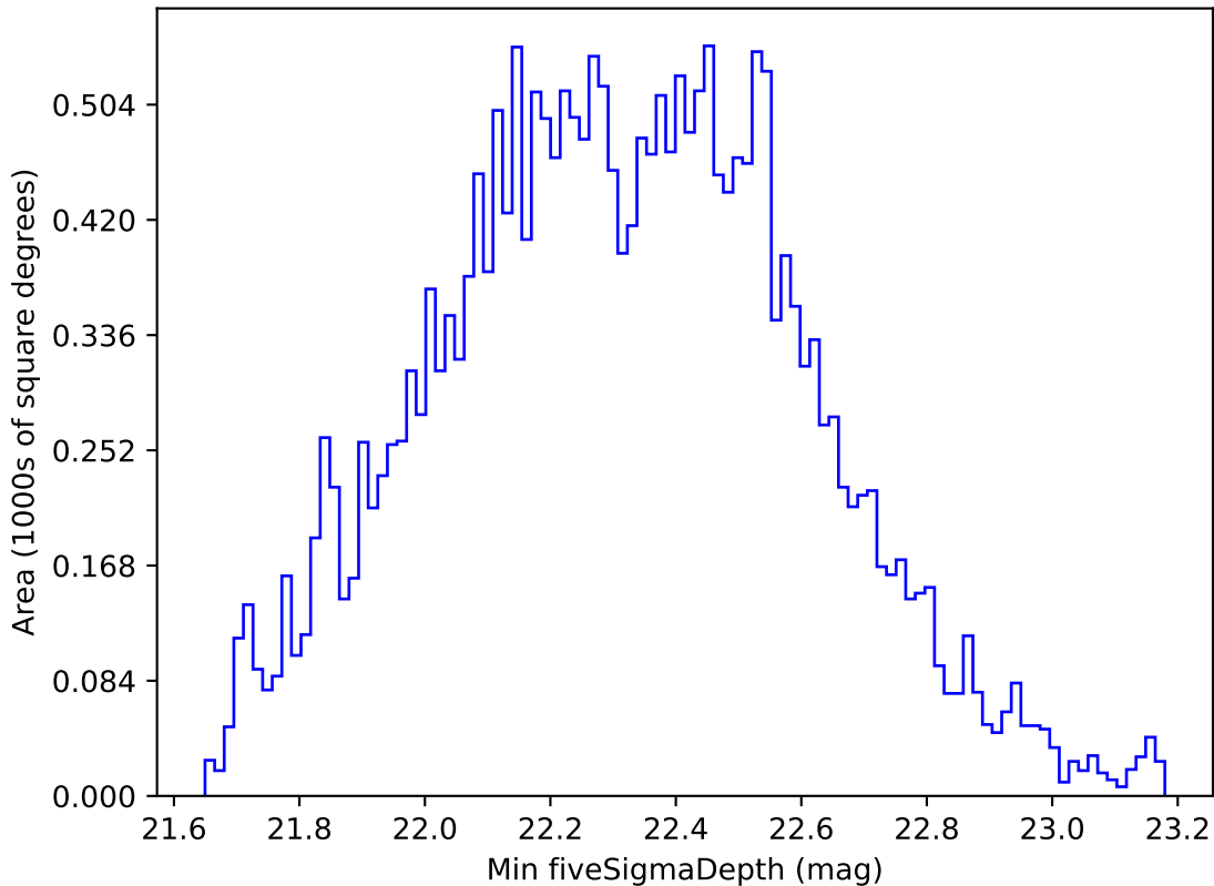
too_elab_r128_d3_ugrizy_v3.4_10yrs All sky u band: Min fiveSigmaDepth
