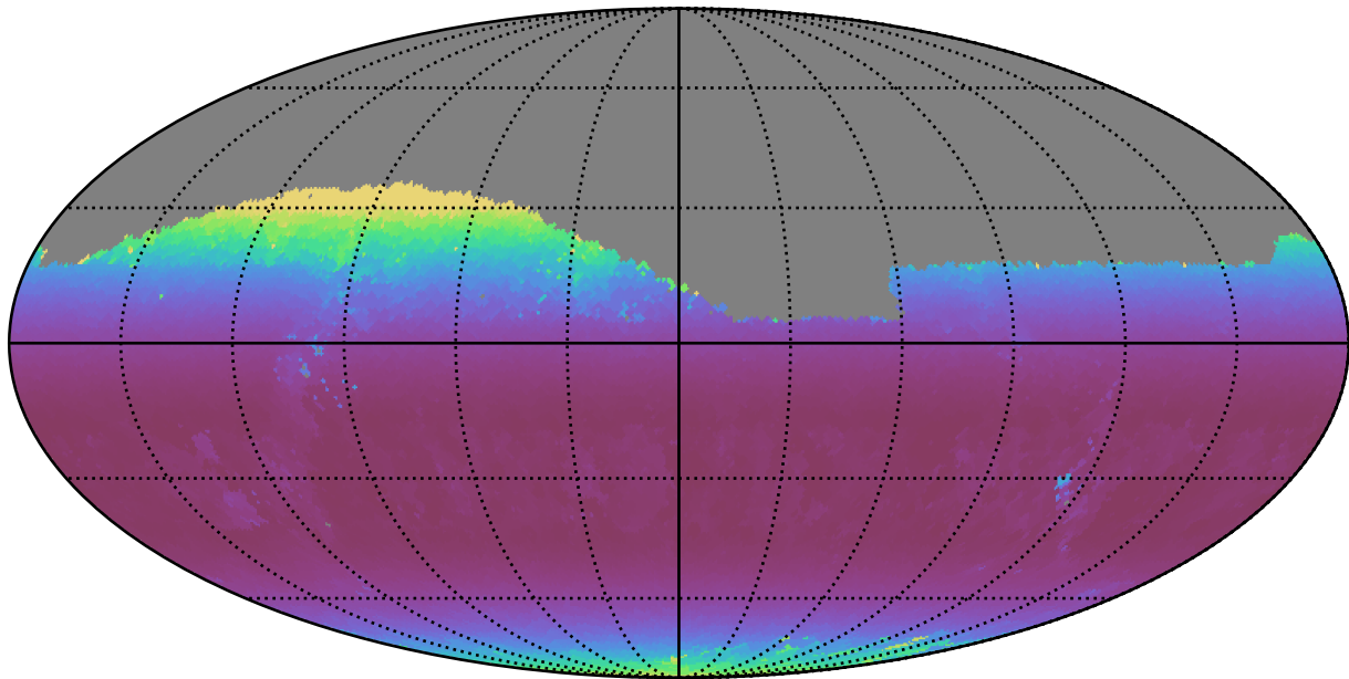
too_elab_r128_d3_ugrizy_v3.4_10yrs Yr 1 z band: Min airmass
