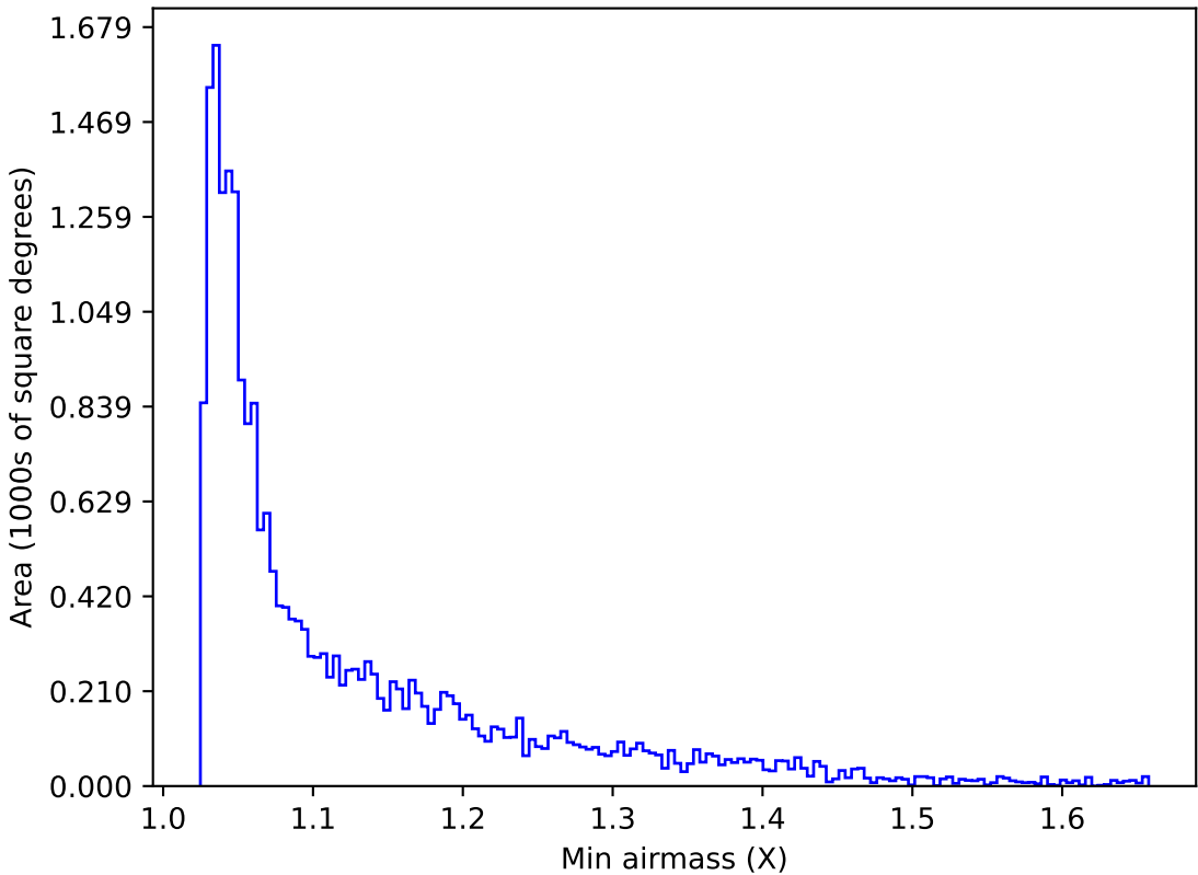
too_elab_r128_d3_ugrizy_v3.4_10yrs Yr 1 y band: Min airmass
