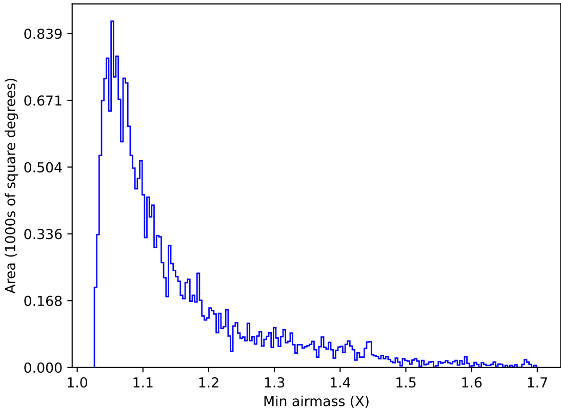
too_elab_r128_d3_ugrizy_v3.4_10yrs Yr 1 u band: Min airmass
