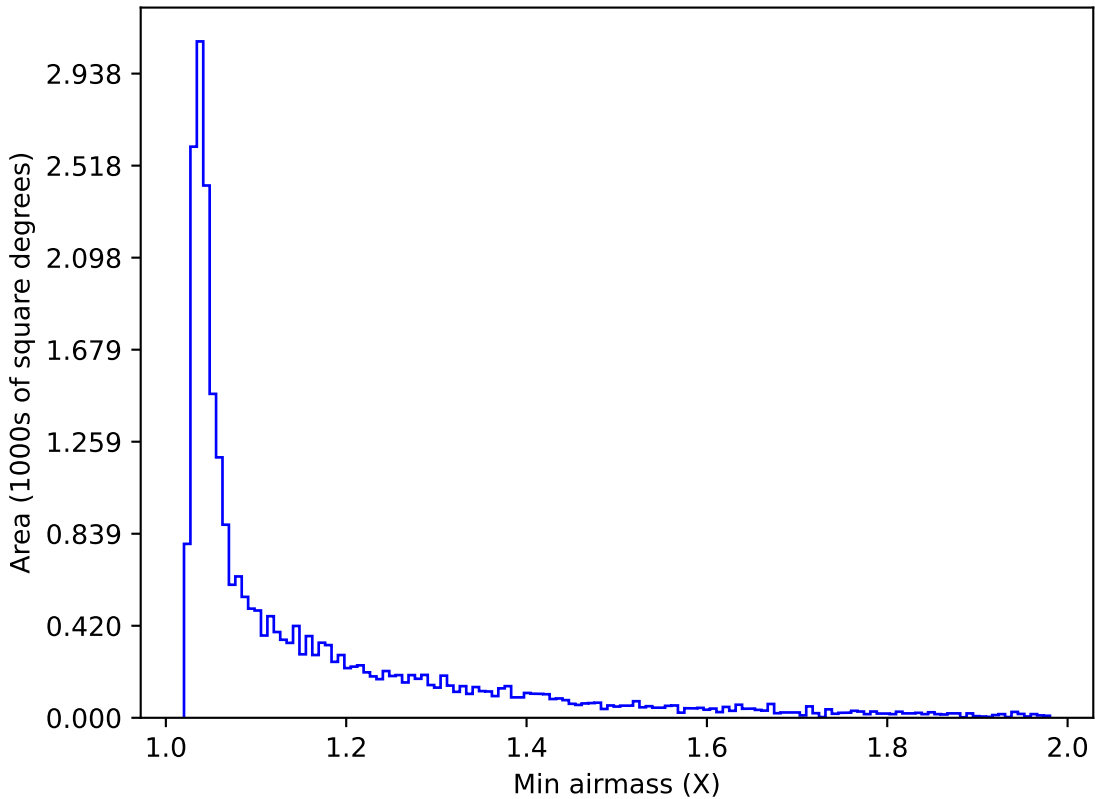
too_elab_r128_d3_ugrizy_v3.4_10yrs Yr 1 i band: Min airmass
