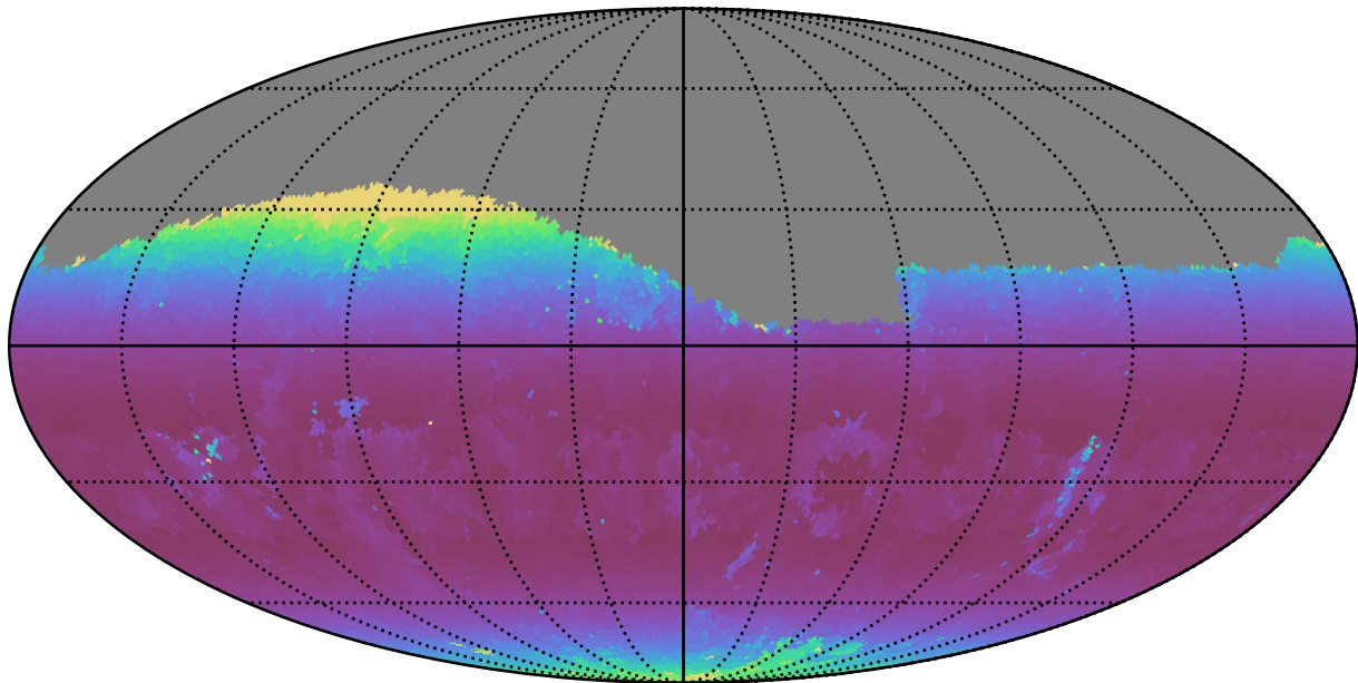
too_elab_r128_d3_ugrizy_v3.4_10yrs Yr 1 g band: Min airmass
