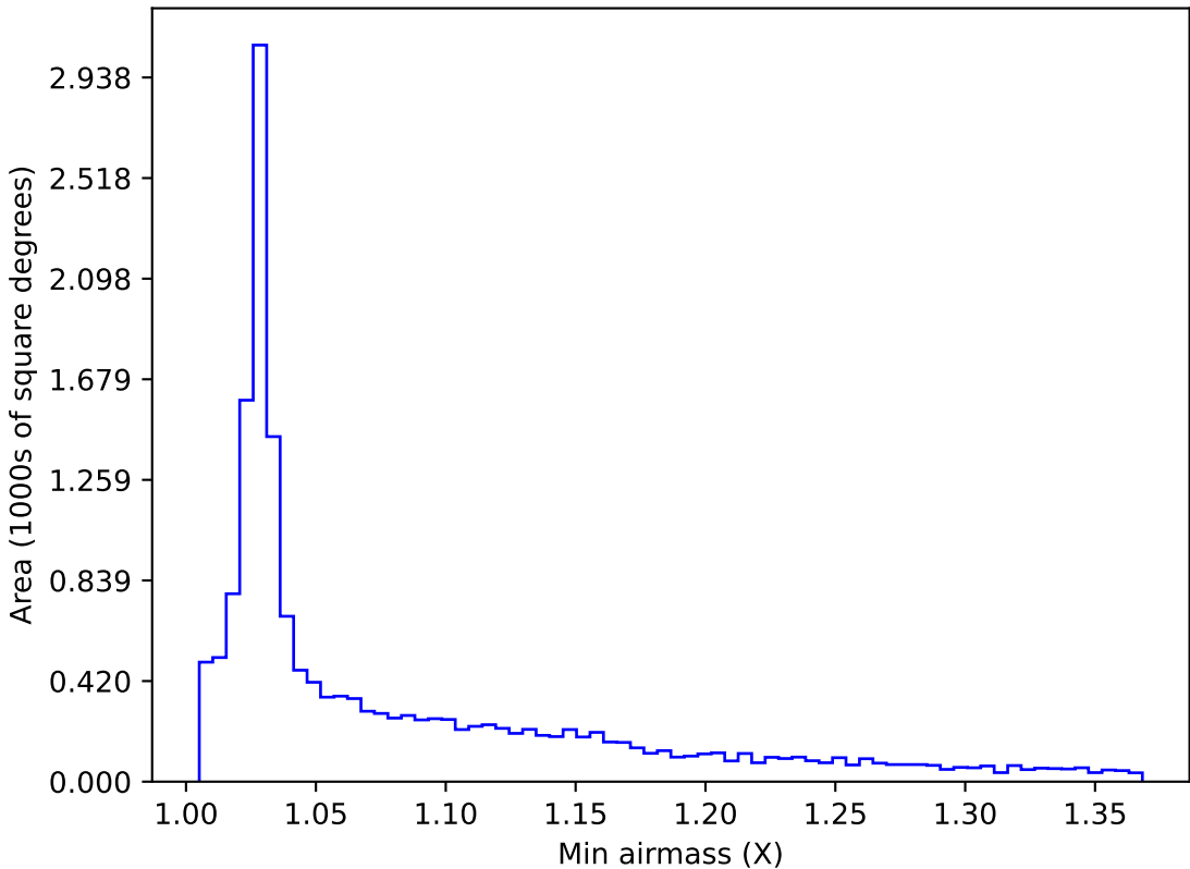
too_elab_r128_d3_ugrizy_v3.4_10yrs WFD z band: Min airmass
