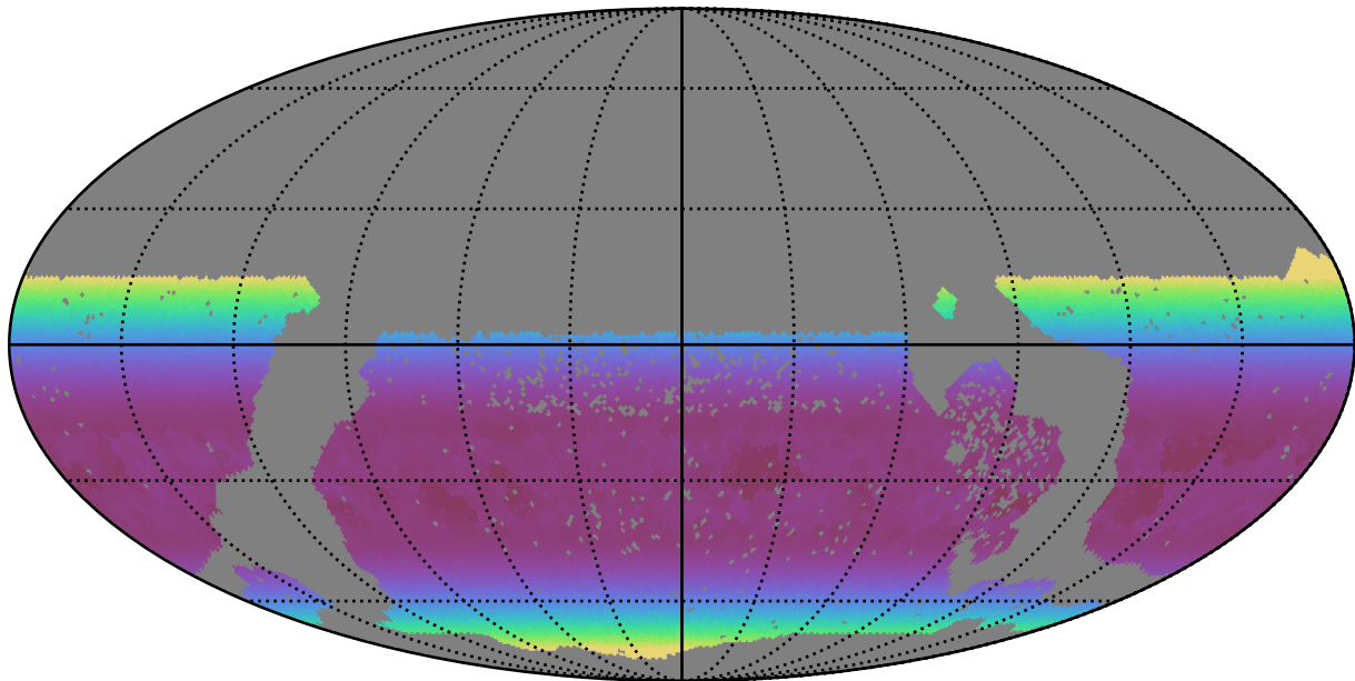
too_elab_r128_d3_ugrizy_v3.4_10yrs WFD y band: Min airmass
