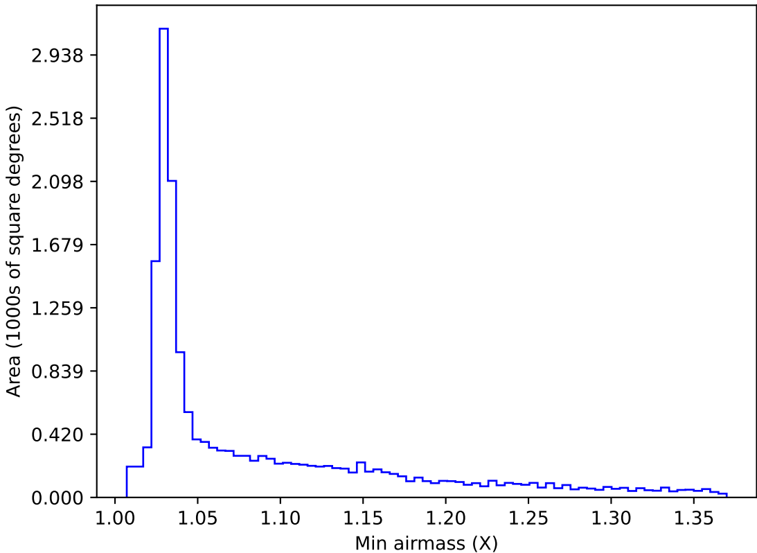
too_elab_r128_d3_ugrizy_v3.4_10yrs WFD y band: Min airmass
