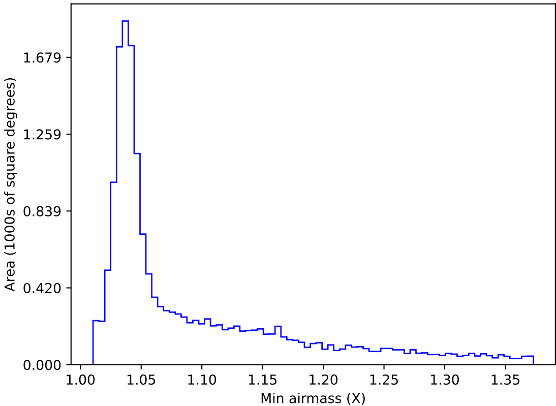
too_elab_r128_d3_ugrizy_v3.4_10yrs WFD u band: Min airmass
