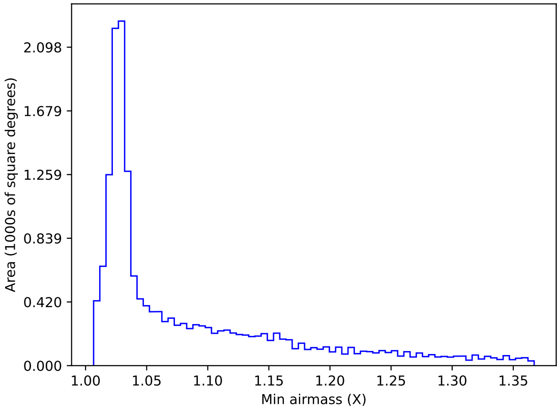
too_elab_r128_d3_ugrizy_v3.4_10yrs WFD r band: Min airmass
