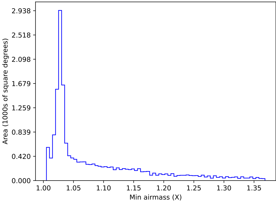
too_elab_r128_d3_ugrizy_v3.4_10yrs WFD i band: Min airmass
