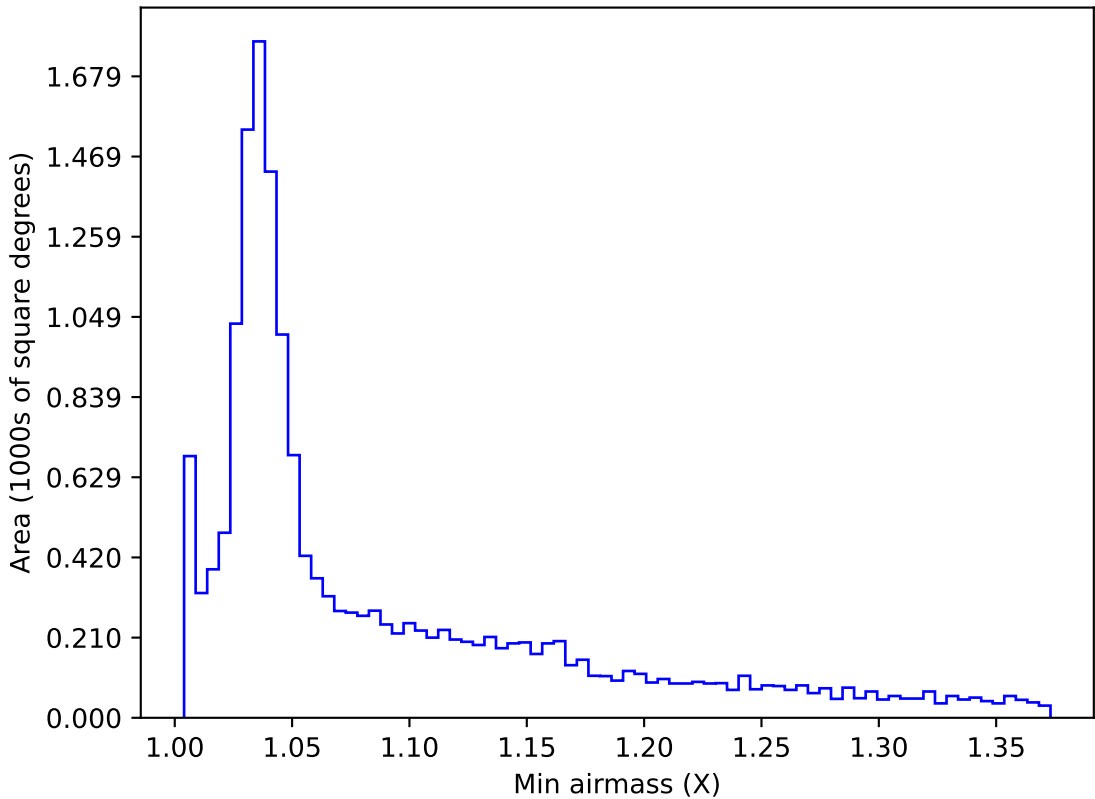
too_elab_r128_d3_ugrizy_v3.4_10yrs WFD g band: Min airmass
