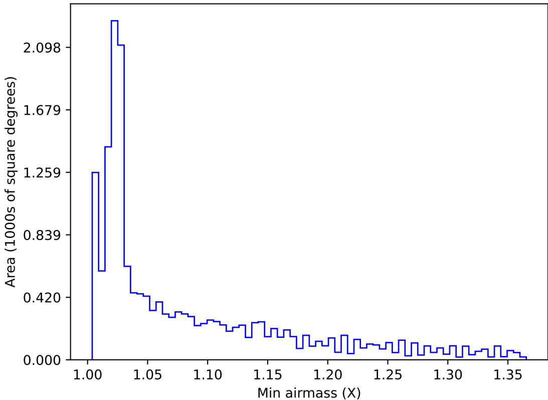
too_elab_r128_d3_ugrizy_v3.4_10yrs WFD all bands: Min airmass
