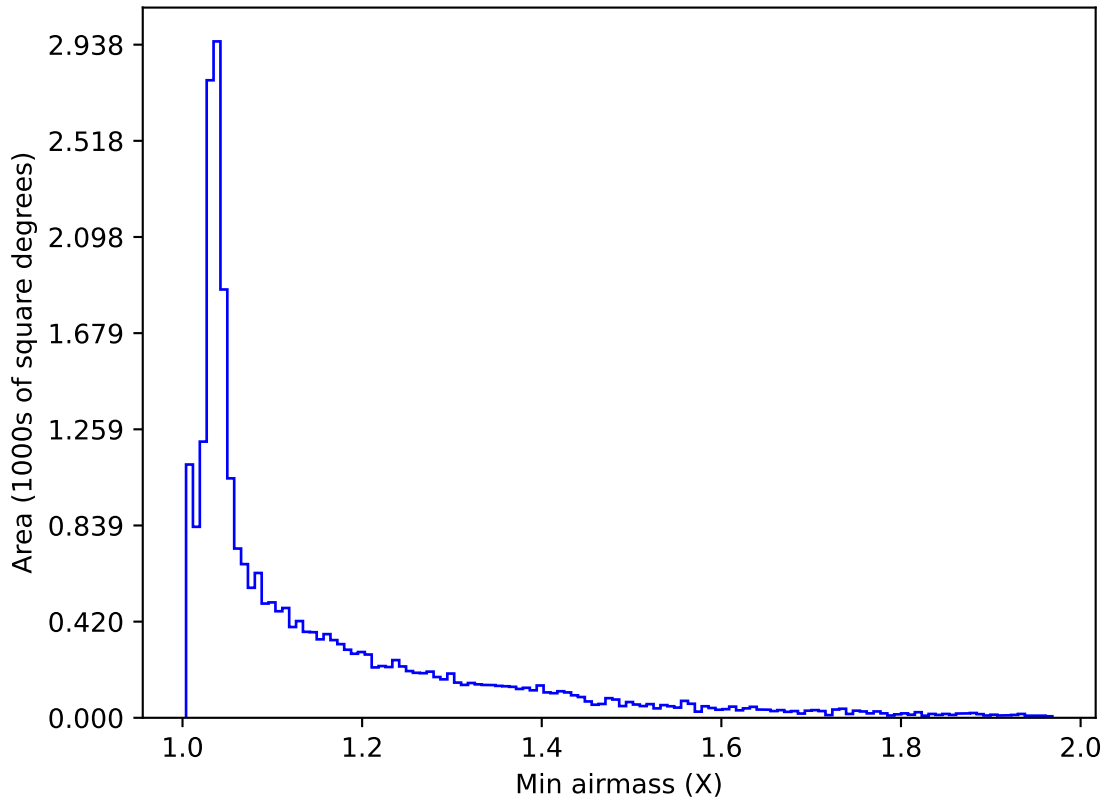
too_elab_r128_d3_ugrizy_v3.4_10yrs All sky g band: Min airmass
