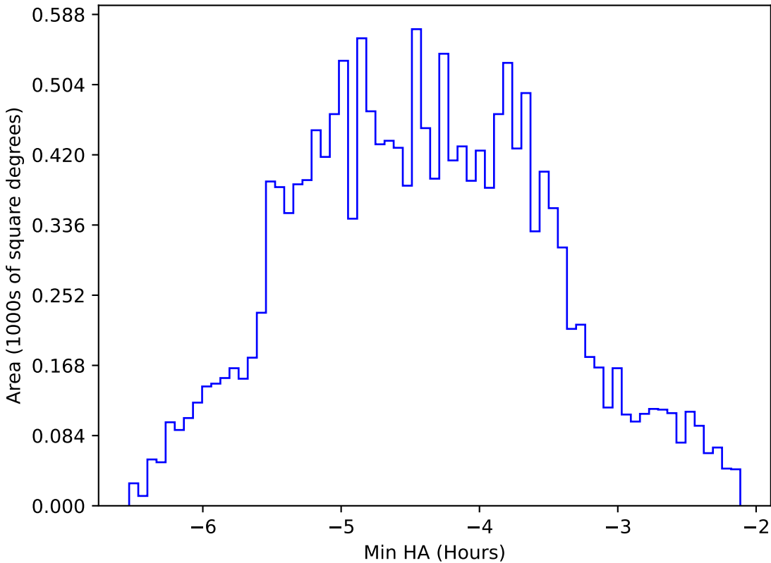
too_elab_r128_d3_ugrizy_v3.4_10yrs WFD z band: Min HA
