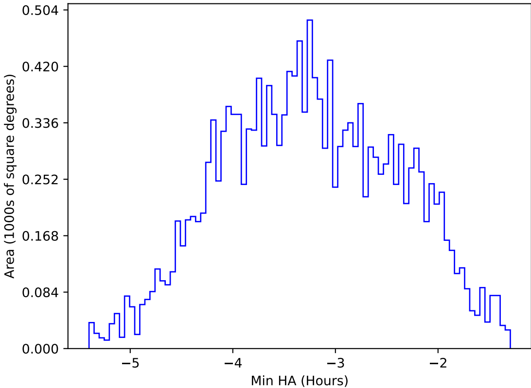
too_elab_r128_d3_ugrizy_v3.4_10yrs WFD u band: Min HA
