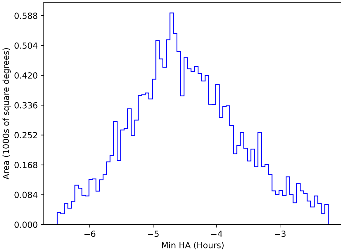
too_elab_r128_d3_ugrizy_v3.4_10yrs WFD i band: Min HA
