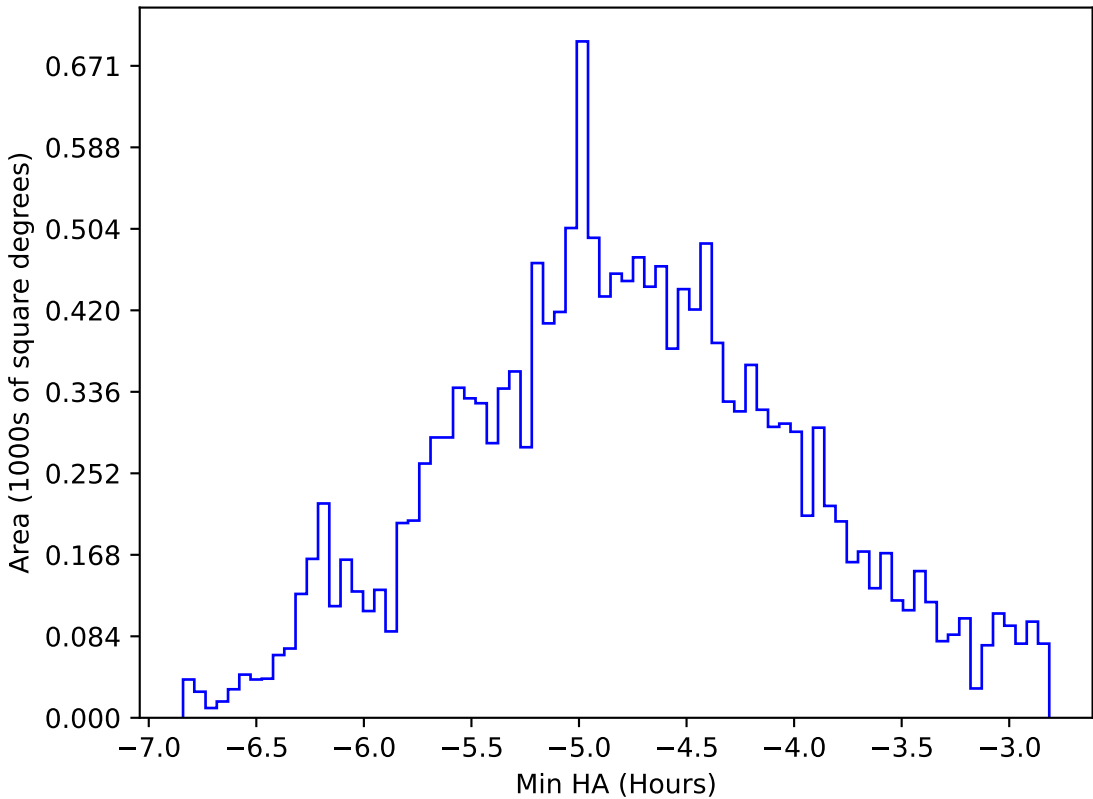
too_elab_r128_d3_ugrizy_v3.4_10yrs WFD all bands: Min HA
