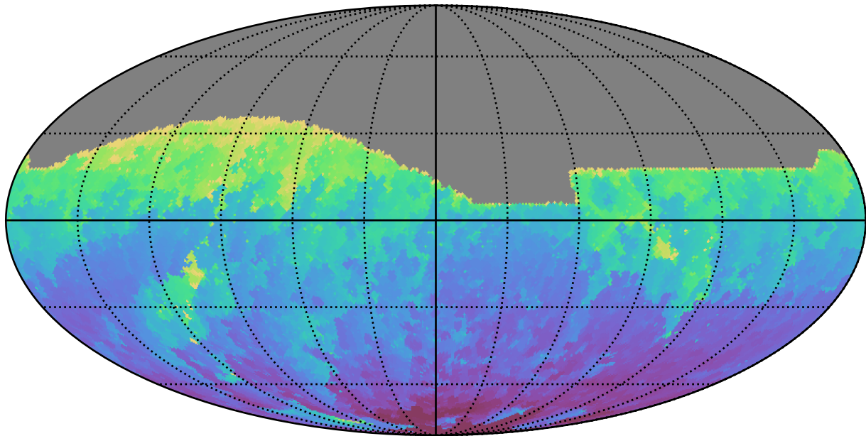
too_elab_r128_d3_ugrizy_v3.4_10yrs All sky z band: Min HA
