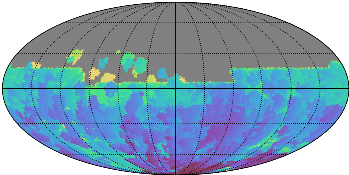
too_elab_r128_d3_ugrizy_v3.4_10yrs All sky u band: Min HA
