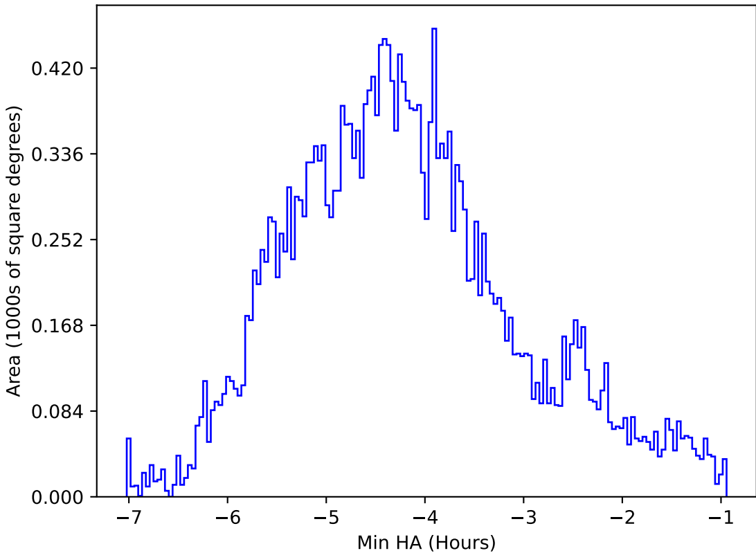
too_elab_r128_d3_ugrizy_v3.4_10yrs All sky r band: Min HA
