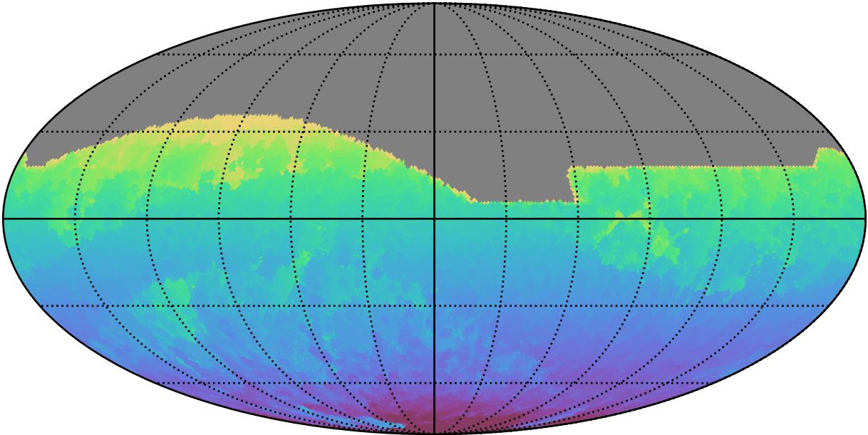
too_elab_r128_d3_ugrizy_v3.4_10yrs All sky all bands: Min HA
