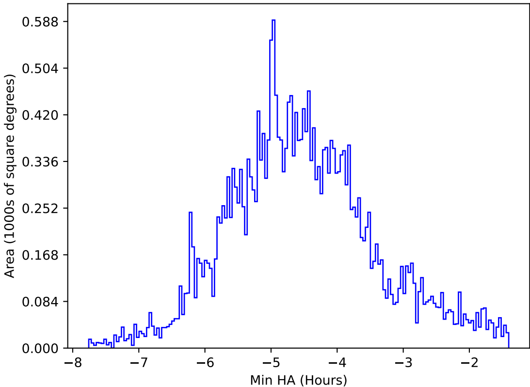
too_elab_r128_d3_ugrizy_v3.4_10yrs All sky all bands: Min HA
