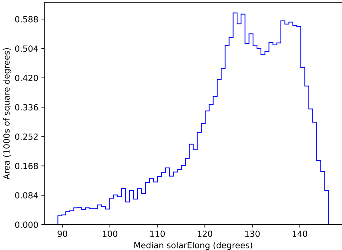
too_elab_r128_d3_ugrizy_v3.4_10yrs WFD z band: Median solarElong
