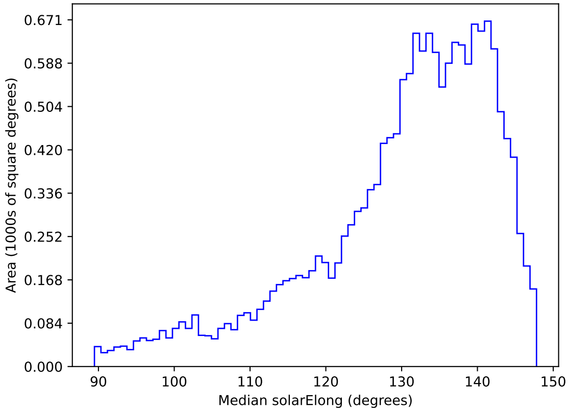
too_elab_r128_d3_ugrizy_v3.4_10yrs WFD y band: Median solarElong
