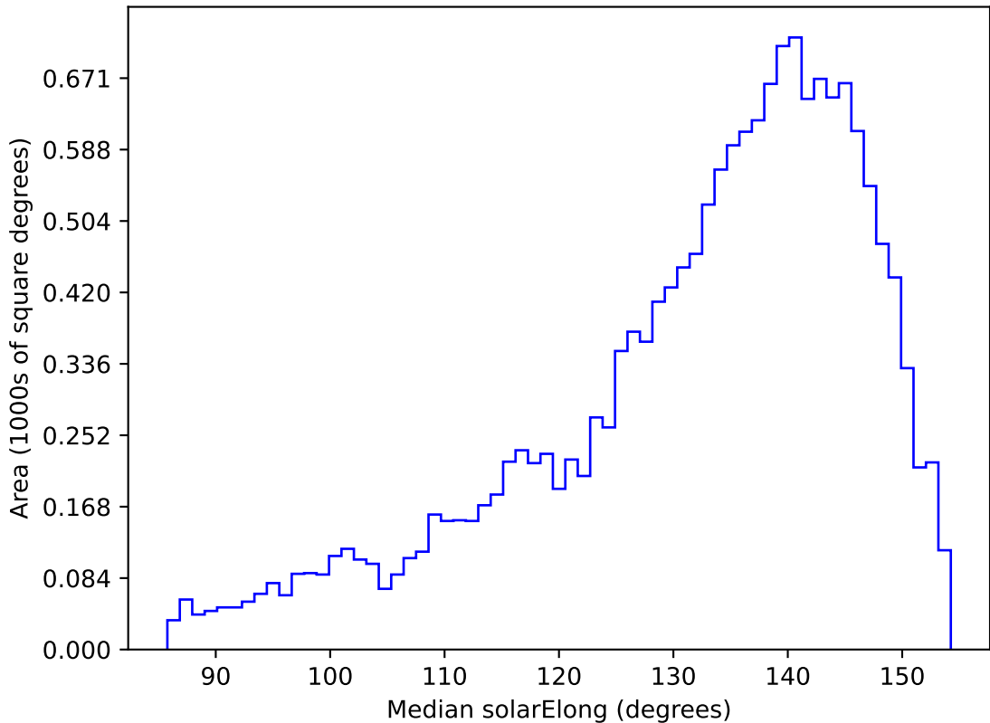
too_elab_r128_d3_ugrizy_v3.4_10yrs WFD u band: Median solarElong
