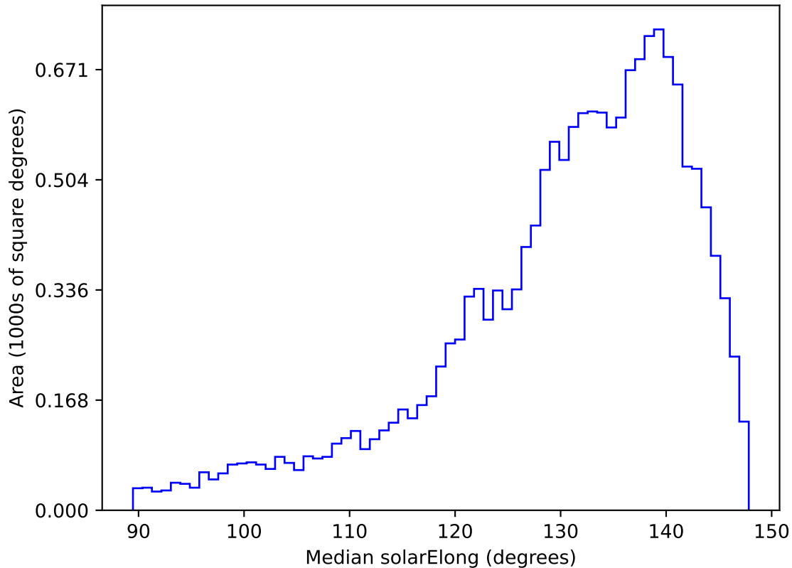
too_elab_r128_d3_ugrizy_v3.4_10yrs WFD r band: Median solarElong
