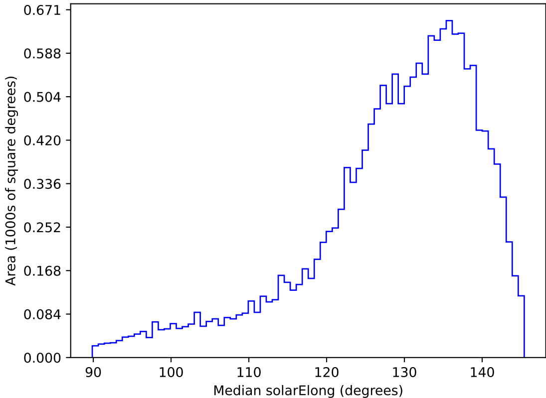
too_elab_r128_d3_ugrizy_v3.4_10yrs WFD i band: Median solarElong
