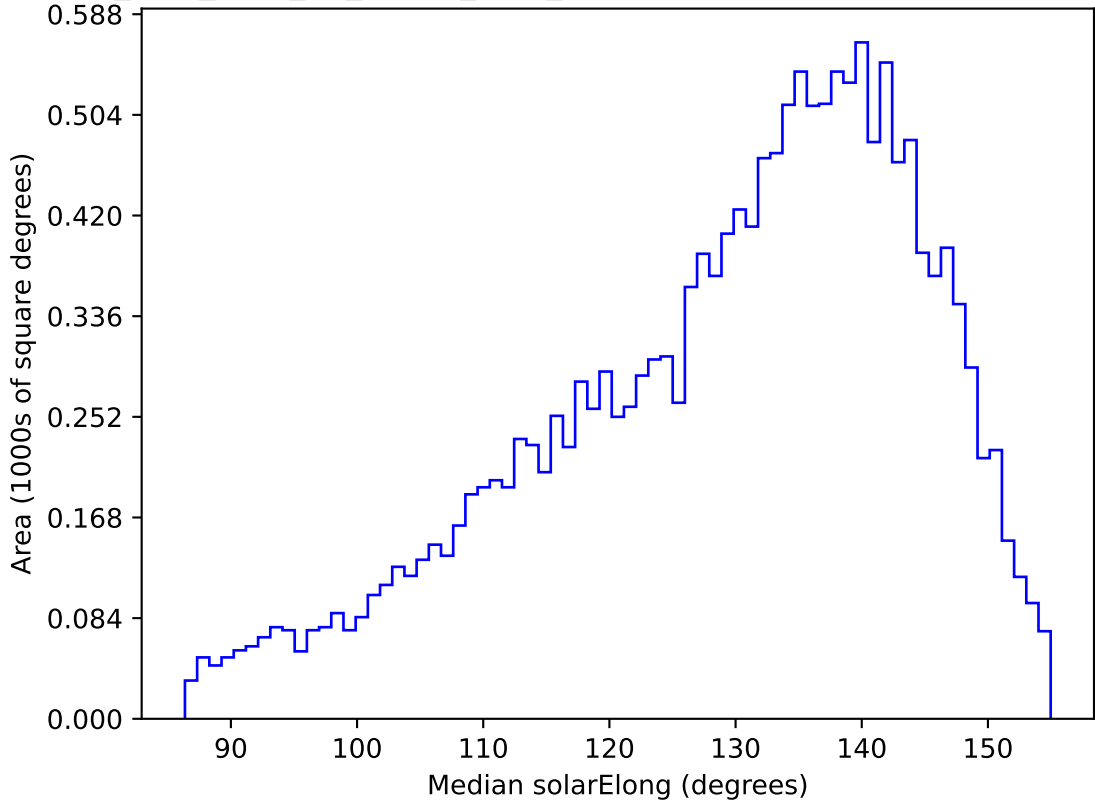
too_elab_r128_d3_ugrizy_v3.4_10yrs WFD g band: Median solarElong
