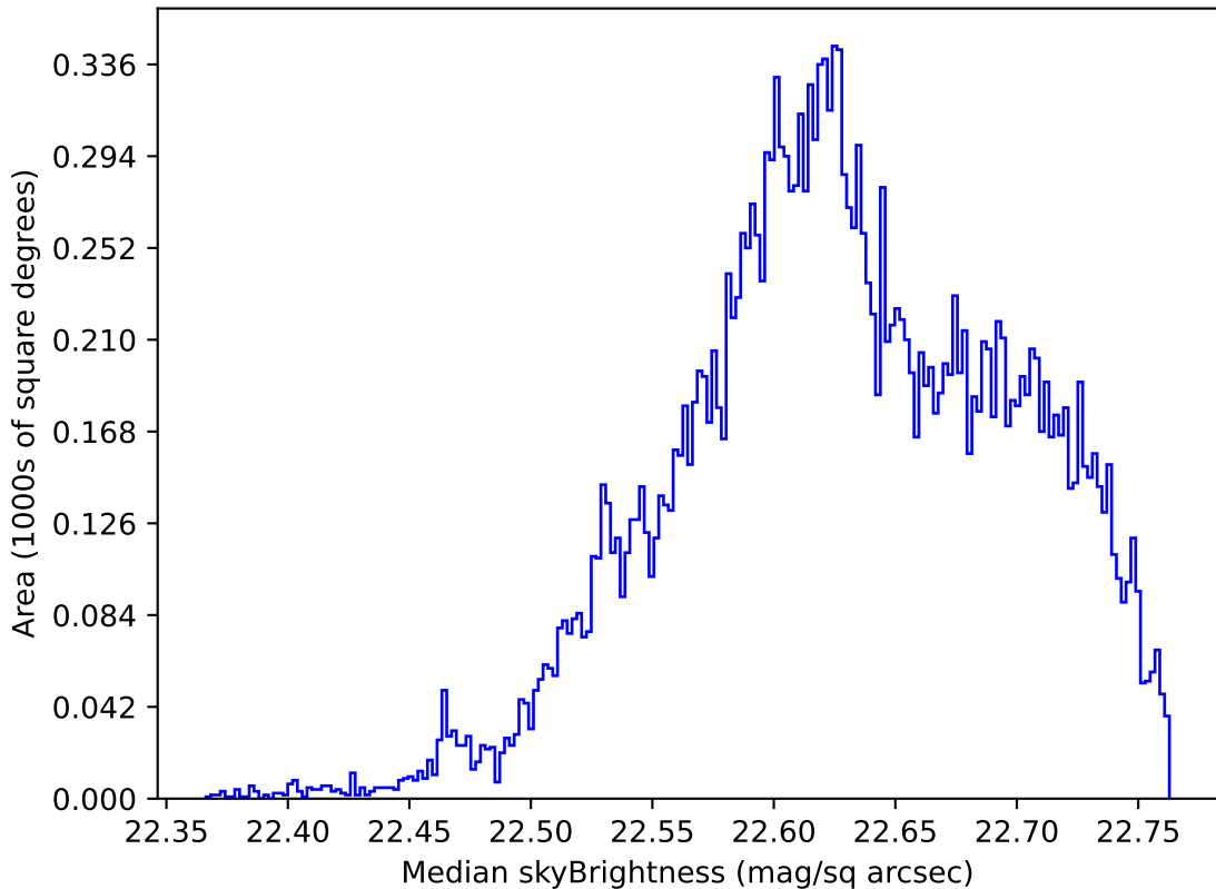
too_elab_r128_d3_ugrizy_v3.4_10yrs Yr 1 u band: Median skyBrightness
