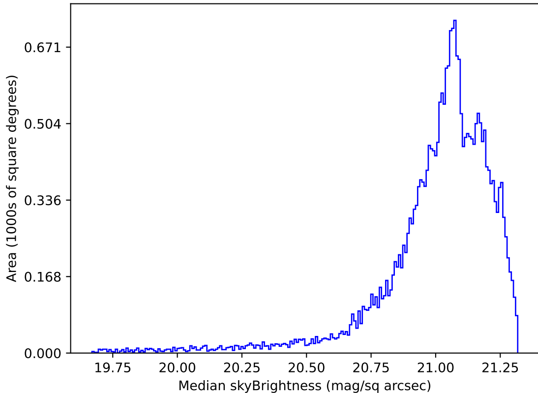
too_elab_r128_d3_ugrizy_v3.4_10yrs Yr 1 r band: Median skyBrightness
