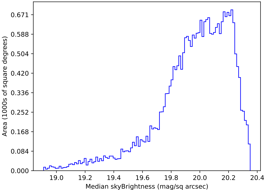
too_elab_r128_d3_ugrizy_v3.4_10yrs Yr 1 i band: Median skyBrightness
