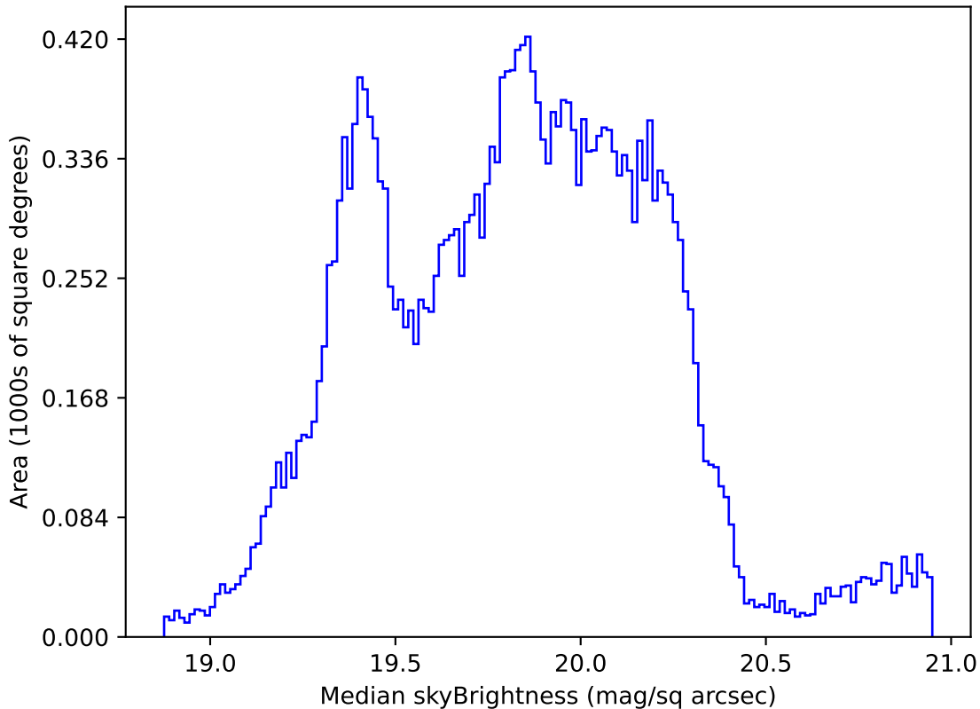
too_elab_r128_d3_ugrizy_v3.4_10yrs Yr 1 all bands: Median skyBrightness
