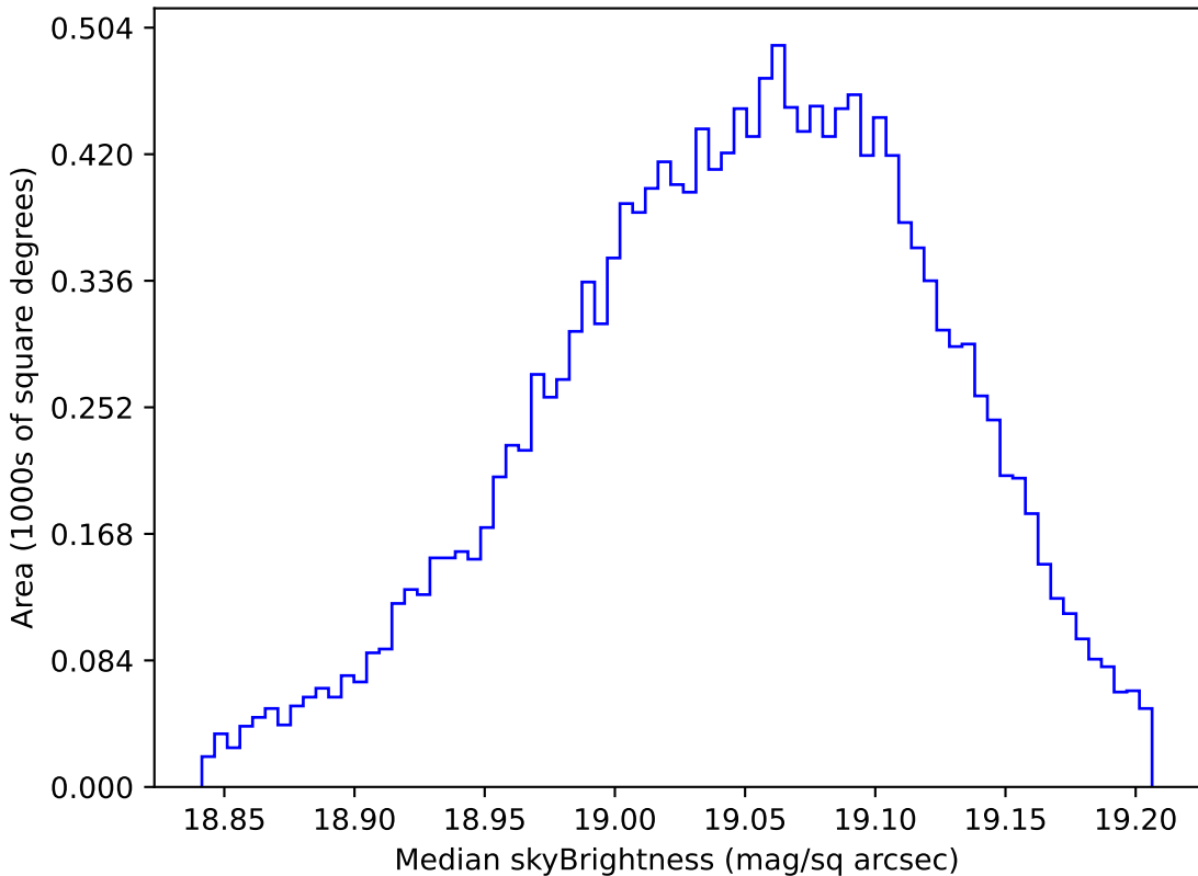
too_elab_r128_d3_ugrizy_v3.4_10yrs WFD z band: Median skyBrightness
