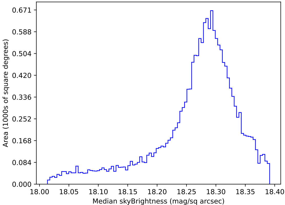
too_elab_r128_d3_ugrizy_v3.4_10yrs WFD y band: Median skyBrightness
