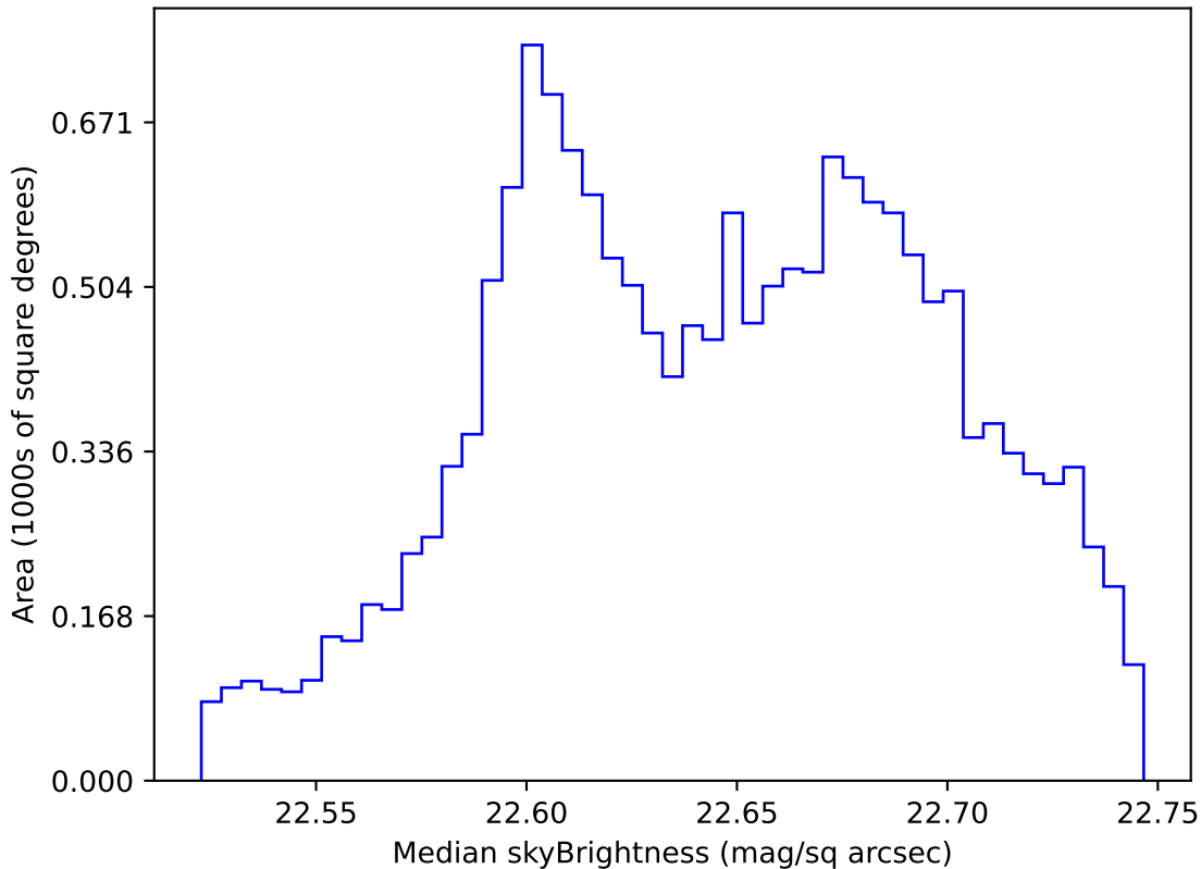
too_elab_r128_d3_ugrizy_v3.4_10yrs WFD u band: Median skyBrightness
