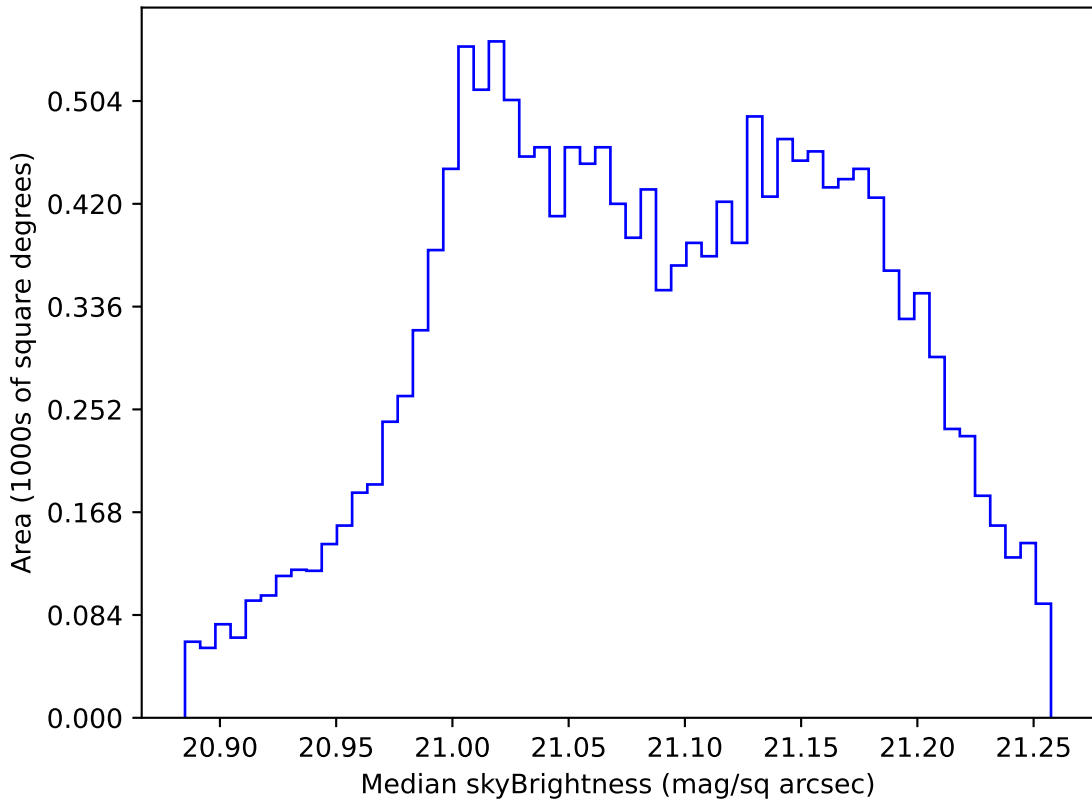
too_elab_r128_d3_ugrizy_v3.4_10yrs WFD r band: Median skyBrightness
