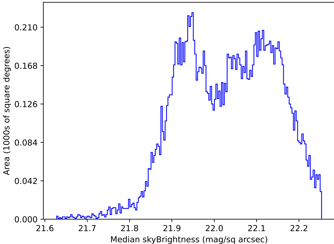
too_elab_r128_d3_ugrizy_v3.4_10yrs WFD g band: Median skyBrightness
