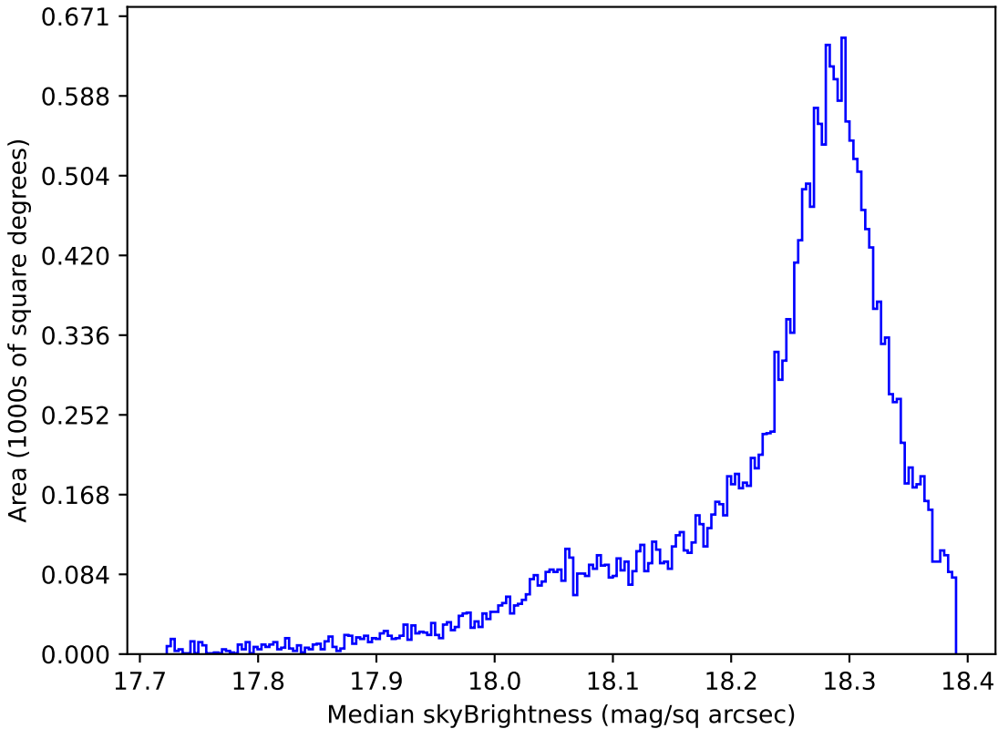
too_elab_r128_d3_ugrizy_v3.4_10yrs All sky y band: Median skyBrightness
