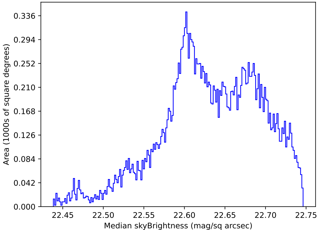
too_elab_r128_d3_ugrizy_v3.4_10yrs All sky u band: Median skyBrightness
